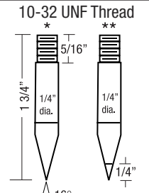
EP0800 Series Electrodes
