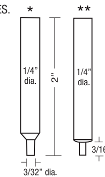
ES0800 Series Electrodes
