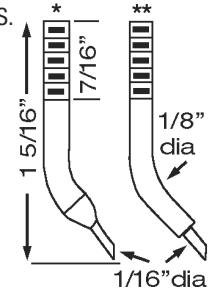
ET0400 Series Electrodes
