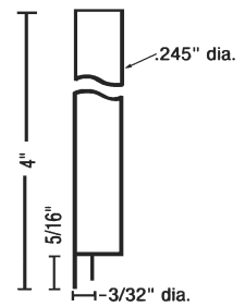
ES0800E Series Electrodes
